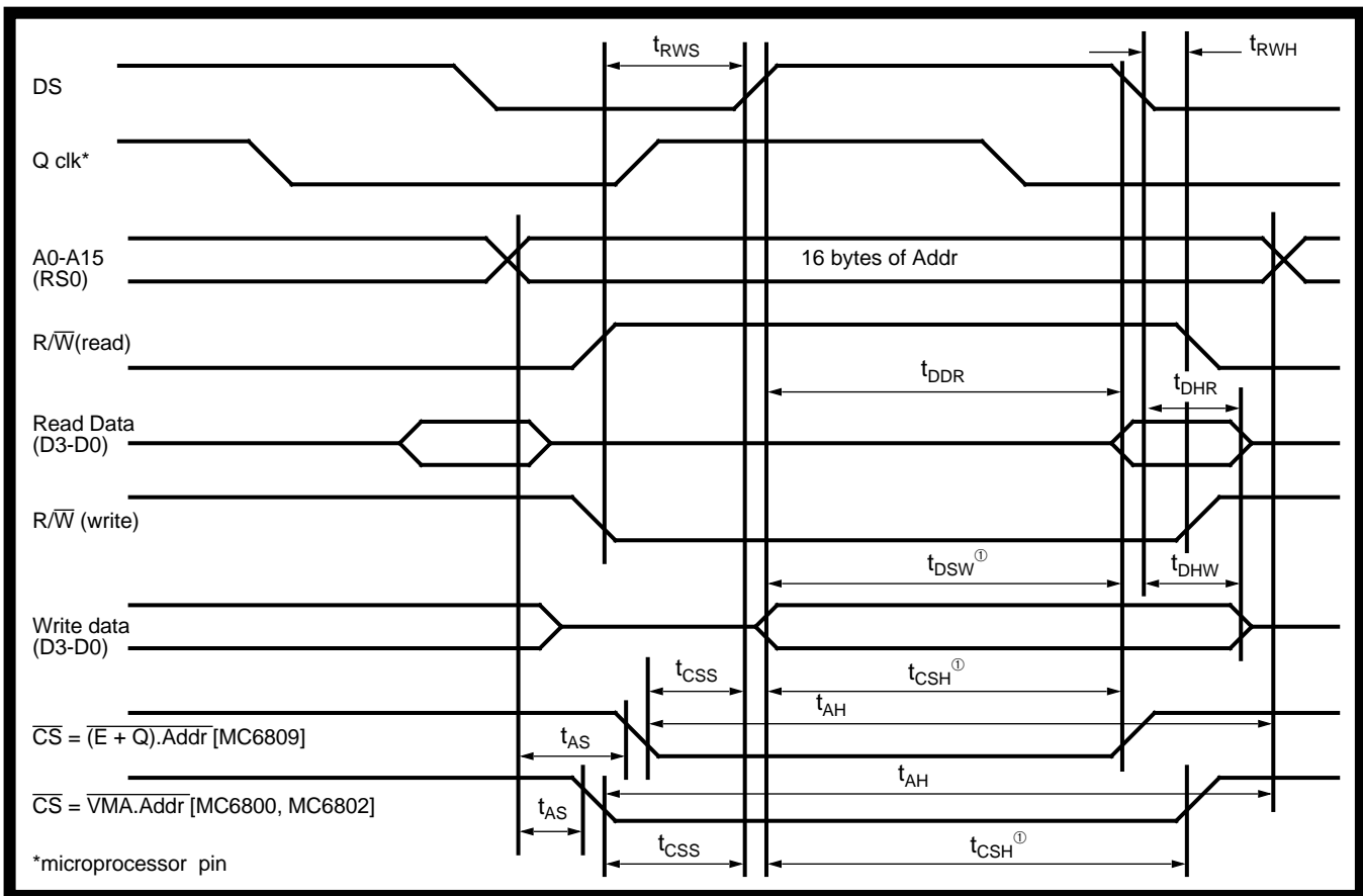
Figure 16 - MC6800/MC6802/MC6809 Timing Diagram
