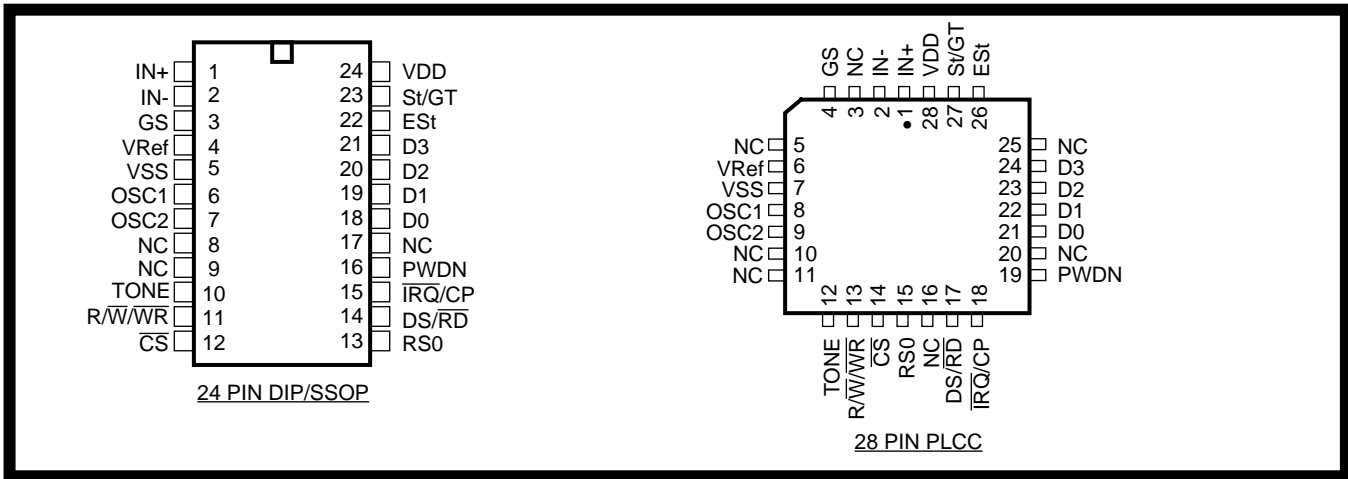
Figure 2 - Pin Connections
